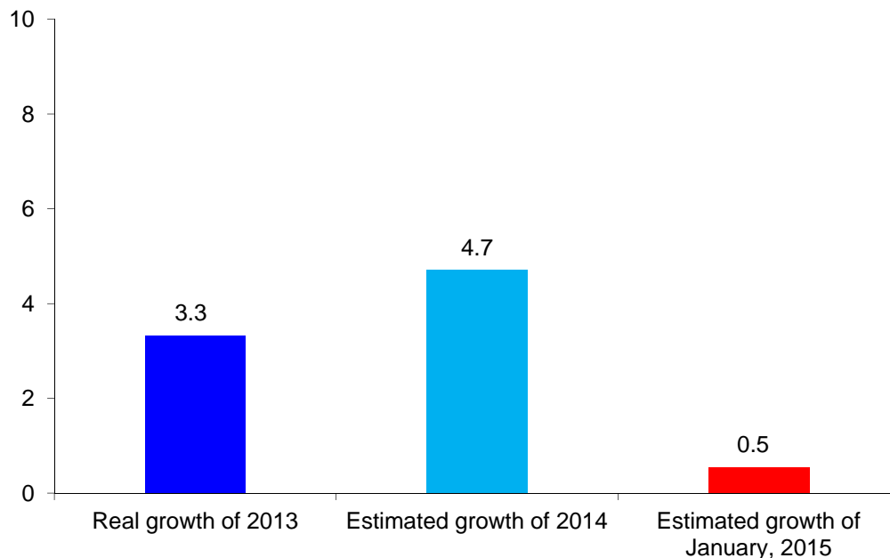
Rapid estimations of economic growth (%)
